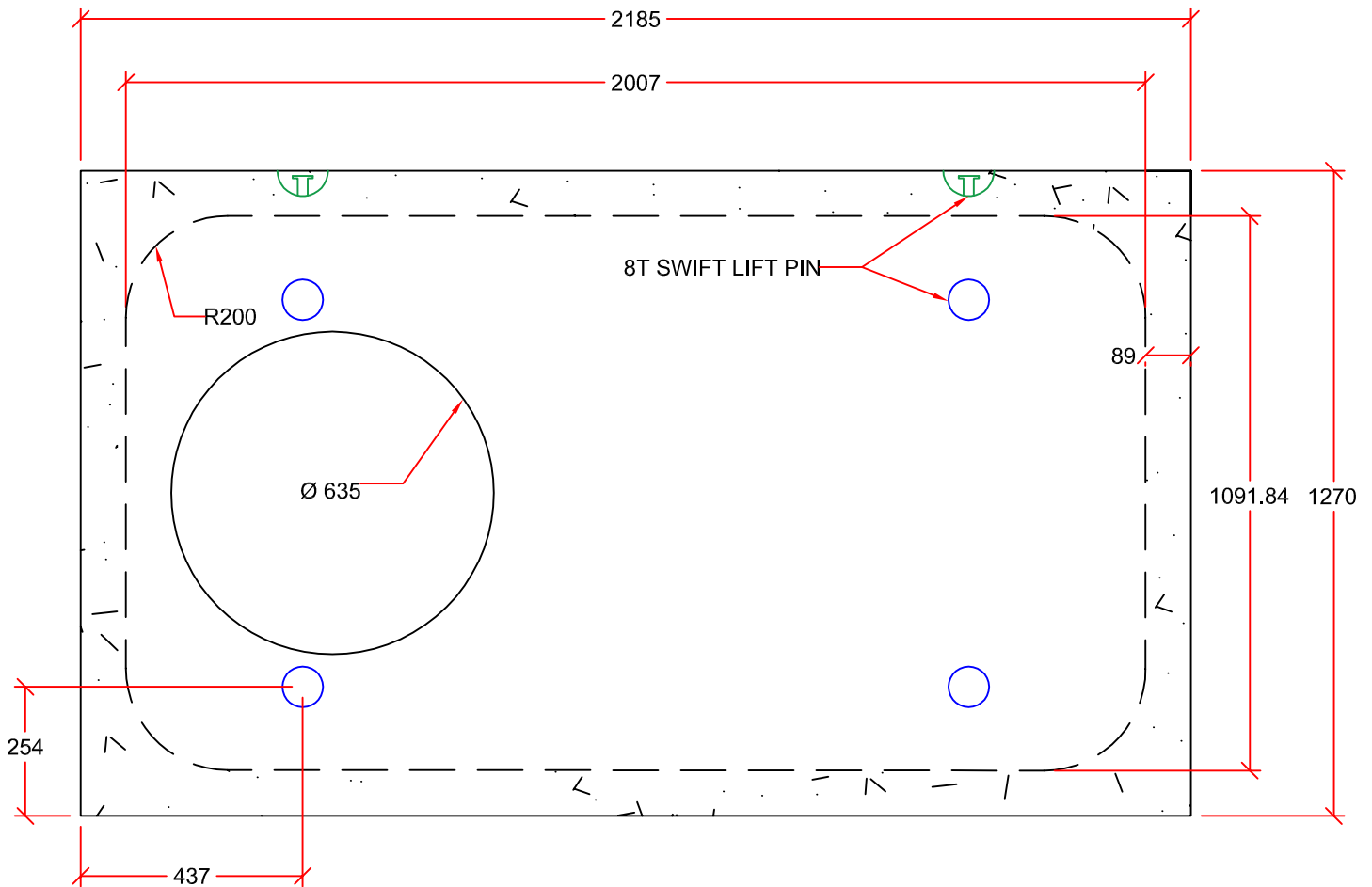
PLAN VIEW
