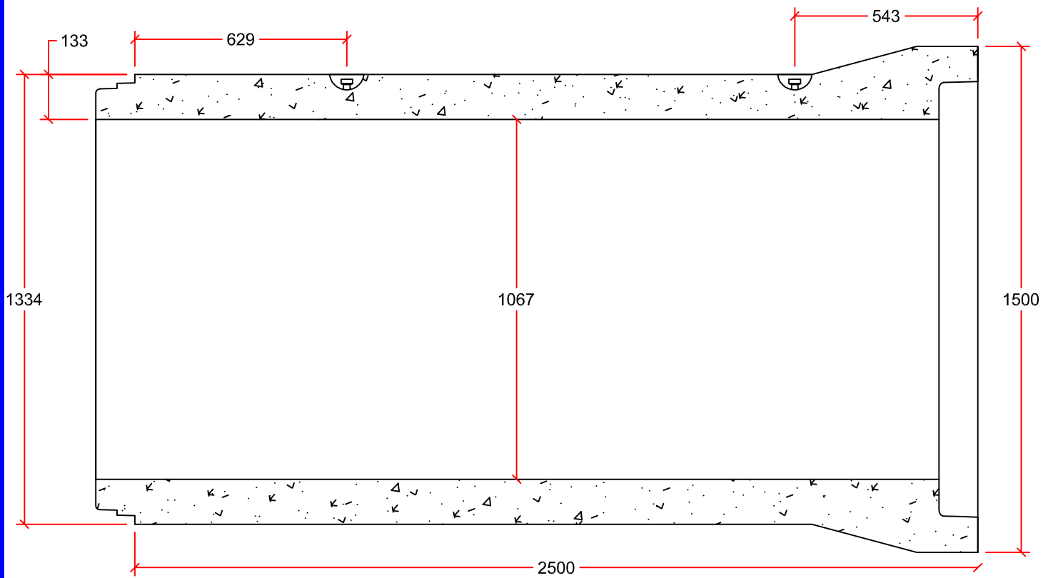
PIPE DETAIL
