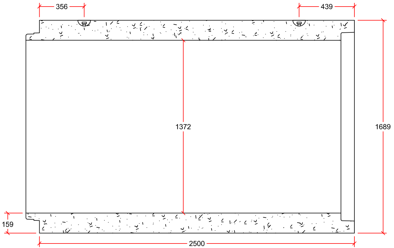
PIPE DETAIL
