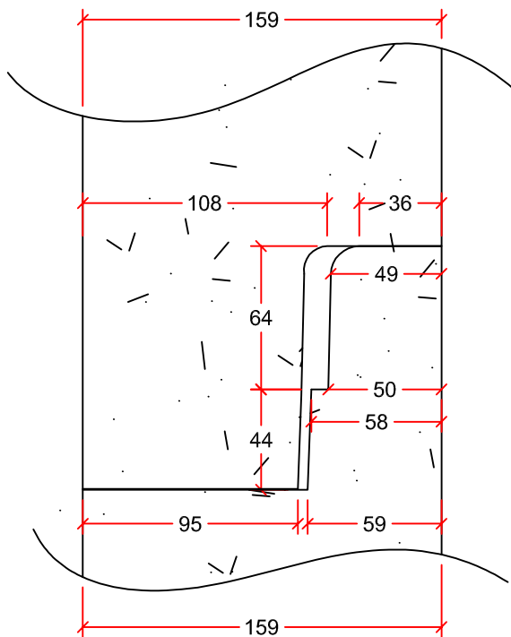
JOINT DETAIL
