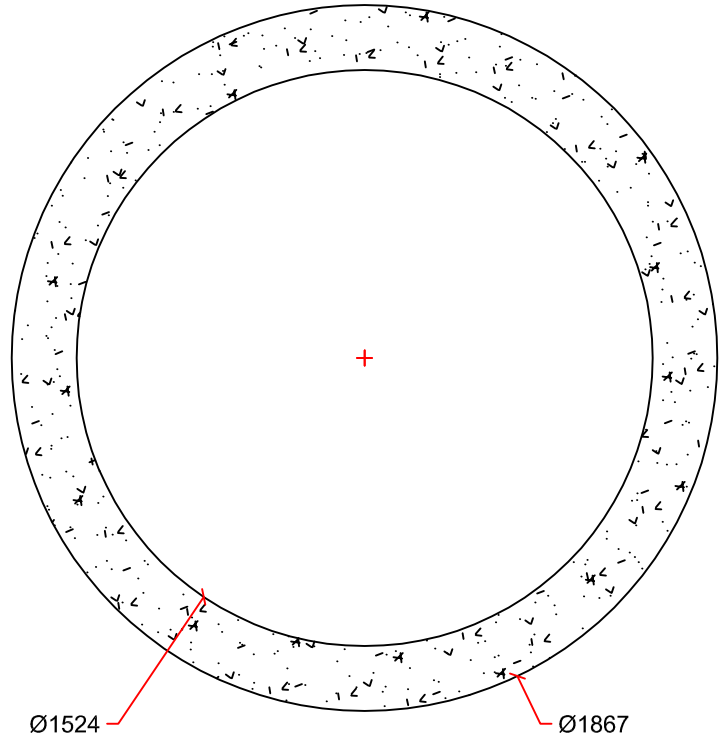
SECTION DETAIL
