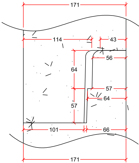
JOINT DETAIL
