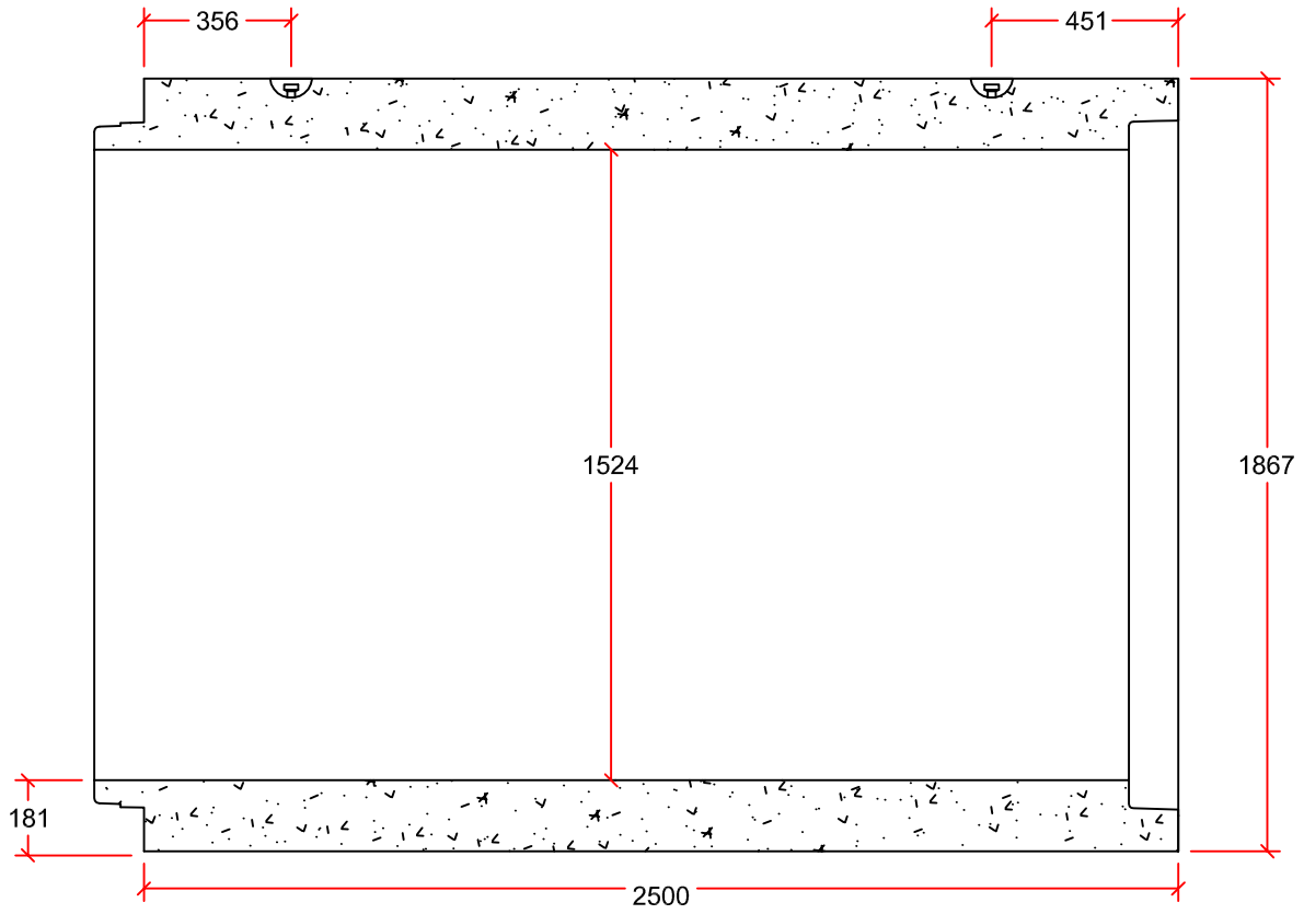
PIPE DETAIL
