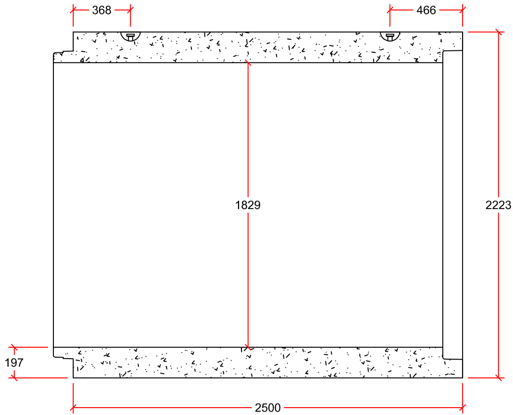
PIPE DETAIL
