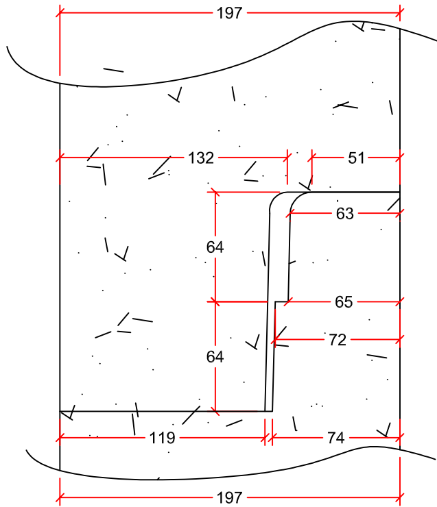
JOINT DETAIL
