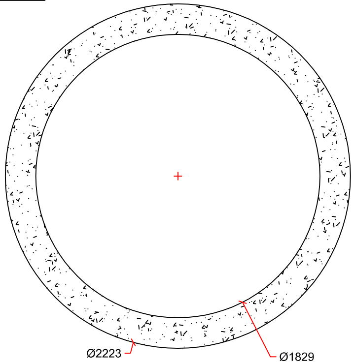
PIPE DETAIL
