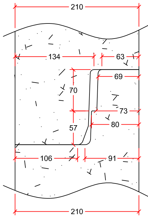
JOINT DETAIL
