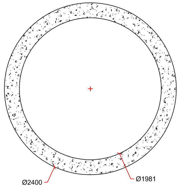
SECTION DETAIL
