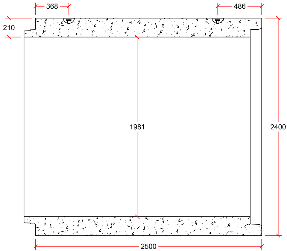
PIPE DETAIL
