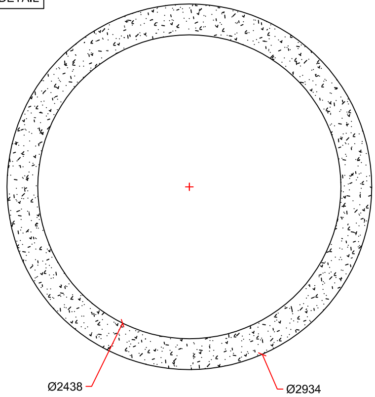
SECTION DETAIL
