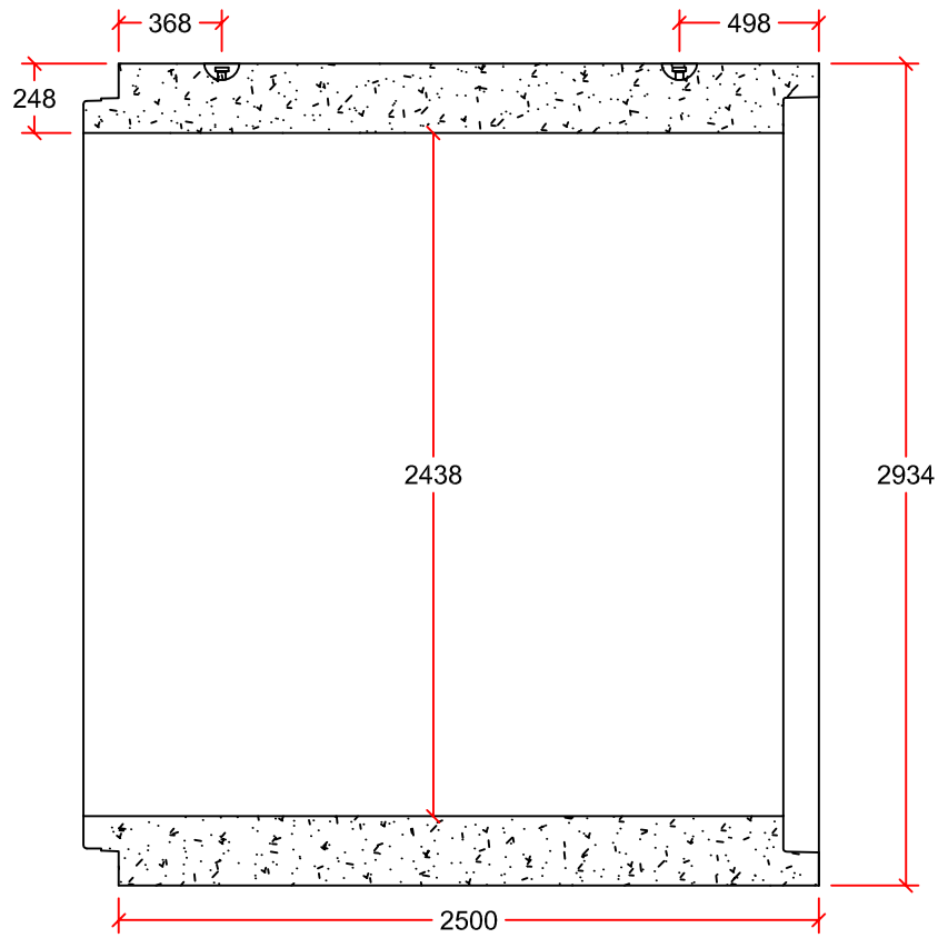
PIPE DETAIL
