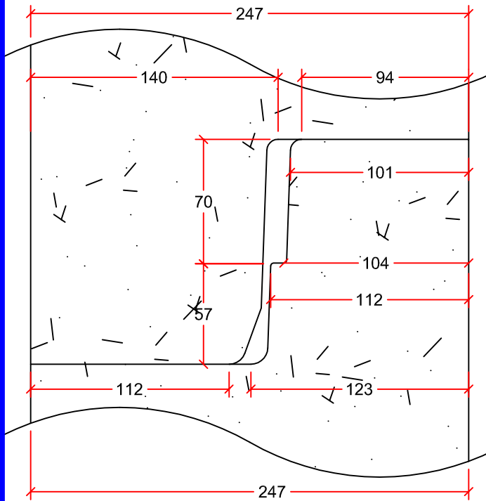
JOINT DETAIL
