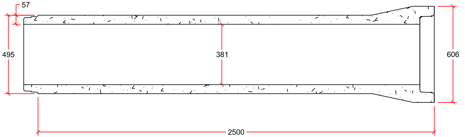
PIPE DETAIL
