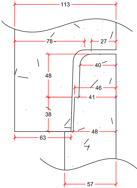
JOINT DETAIL
