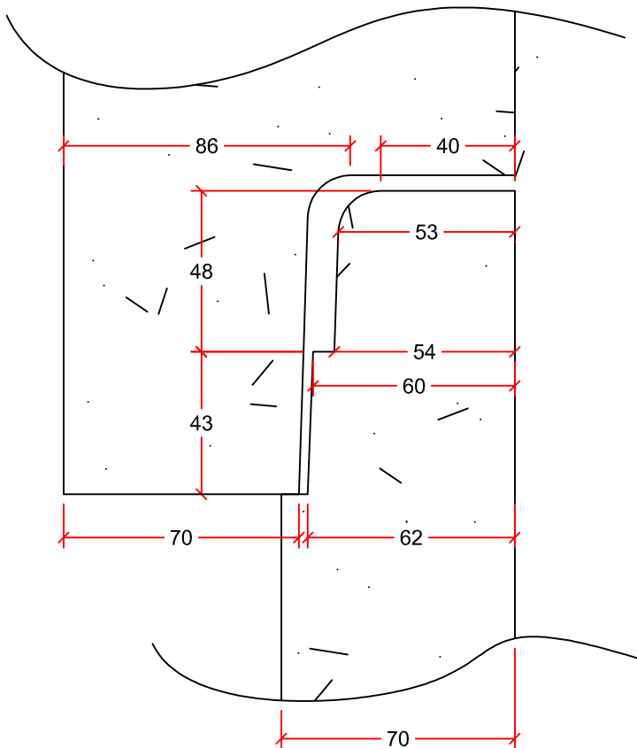
JOINT DETAIL
