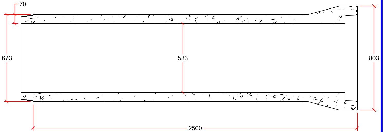
PIPE DETAIL
