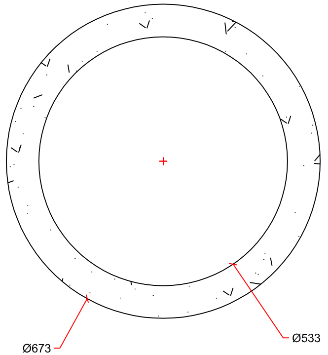
SECTION DETAIL
