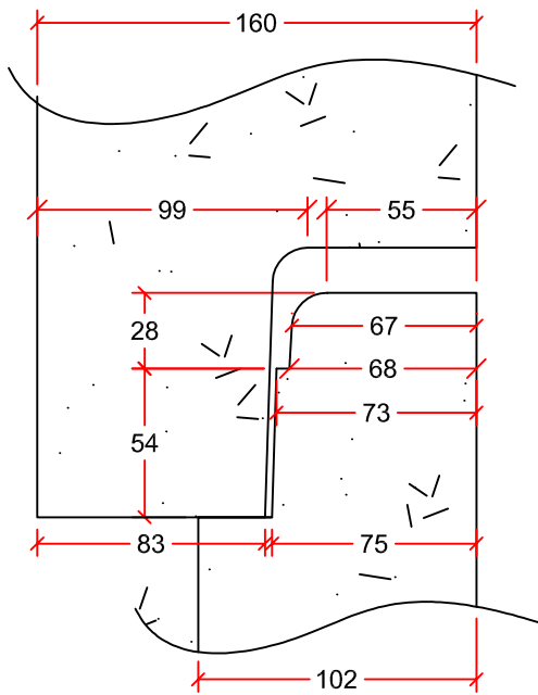
JOINT DETAIL
