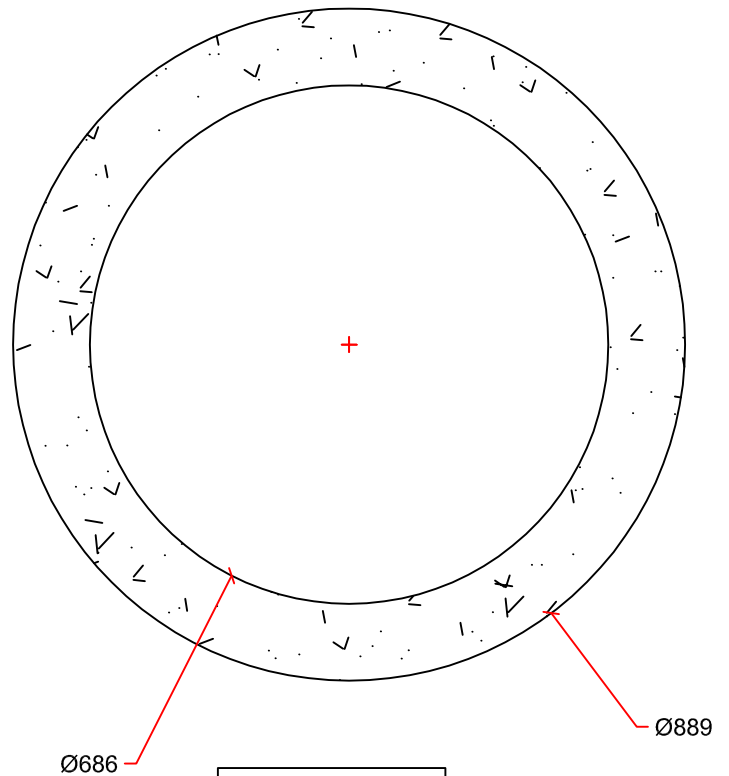
SECTION DETAIL
