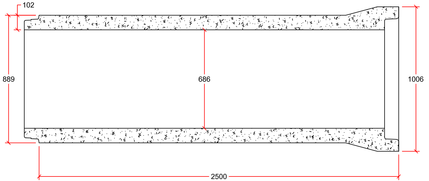
PIPE DETAIL
