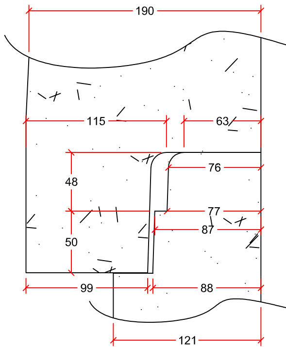
JOINT DETAIL
