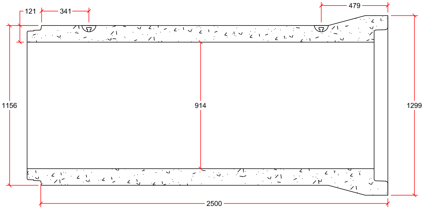
PIPE DETAIL
