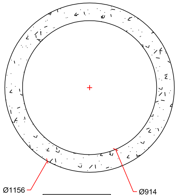
SECTION DETAIL
