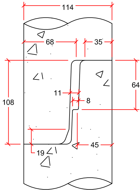
JOINT DETAIL
