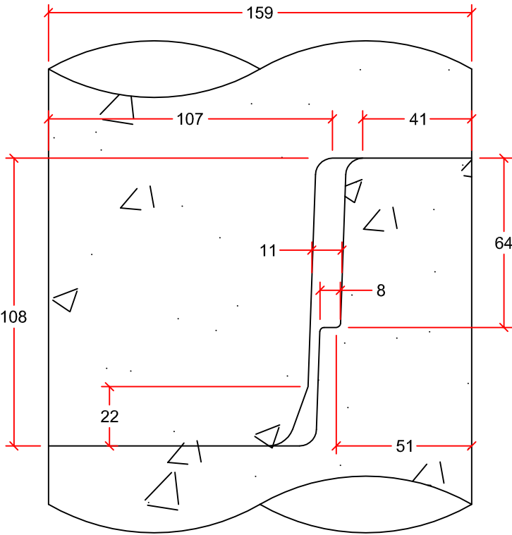
JOINT DETAIL
