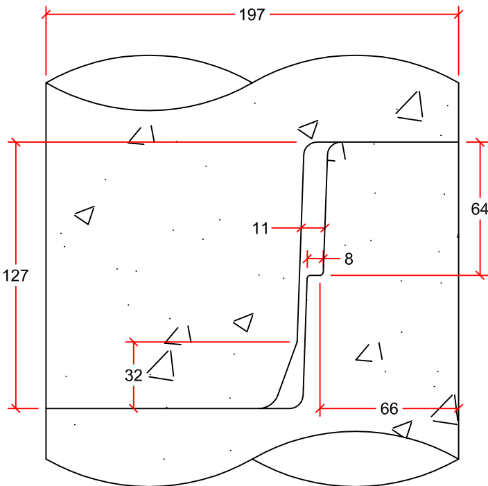
JOINT DETAIL
