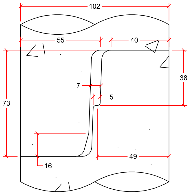
JOINT DETAIL
